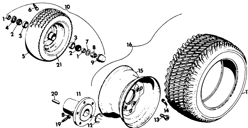
FRONT & REAR WHEEL ASSEMBLIES
